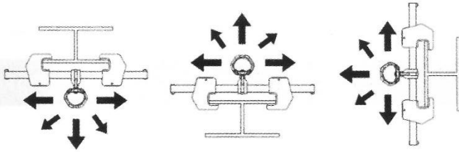
Figure 3: Loading Directions
